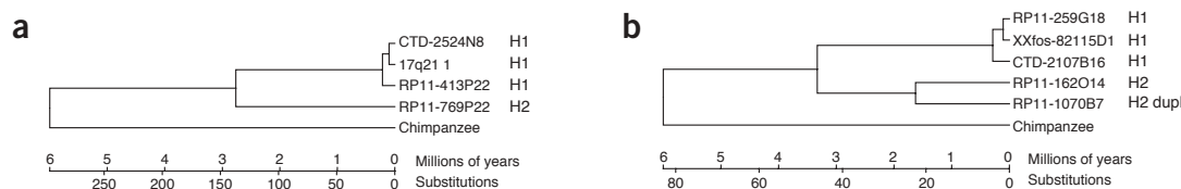
Figure 2 The sequence divergence of the H1 and H2 lineages. (a) A maximum parsimony tree based on substitutions identified in full sequences from clones spanning a 77-kb region containing the first two exons and introns of MAPT (44.444005–44.520949 Mb in Build 34). (b) A maximum parsimony tree based on 32-kb clone sequences for a region that is present on both the H1 and H2 lineages but is duplicated (dupl) in the RP11 H2 chromosome (44.730628–44.762592 Mb in Build 34). The sequence divergence between the H1 and H2 lineages in b is 0.2894%, indicating a coalescent age of close to 3 million years, with the age of the duplication event in the H2 lineage estimated at ~1.5 million years and a divergence among H1 sequences of 0.0167%. Both trees show an unusually deep divergence between the H1 and H2 lineages relative to the overall sequence divergence between humans and chimpanzees in this region (see Supplementary Fig. 5 online for a 5-kb sliding-window analysis of sequence divergence in the two sequence regions). The age estimation for the split between the H1 and H2 lineages is dependent on a number of assumptions, such as neutral evolution and equivalent mutation rates along all branches. The roughly equal divergence of the H1 and H2 lineages from the chimpanzee sequence indicates that selection has at least not differentially affected the accumulation of mutations in the H1 and H2 lineages.
